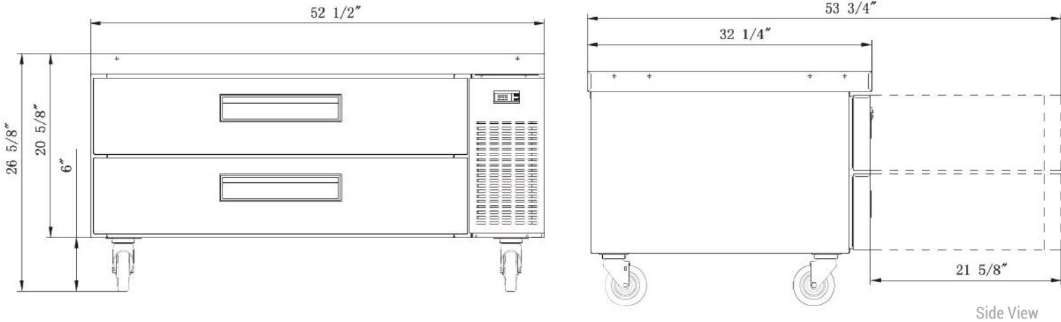
Side View
