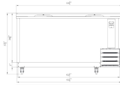
DHBC65 Front View
